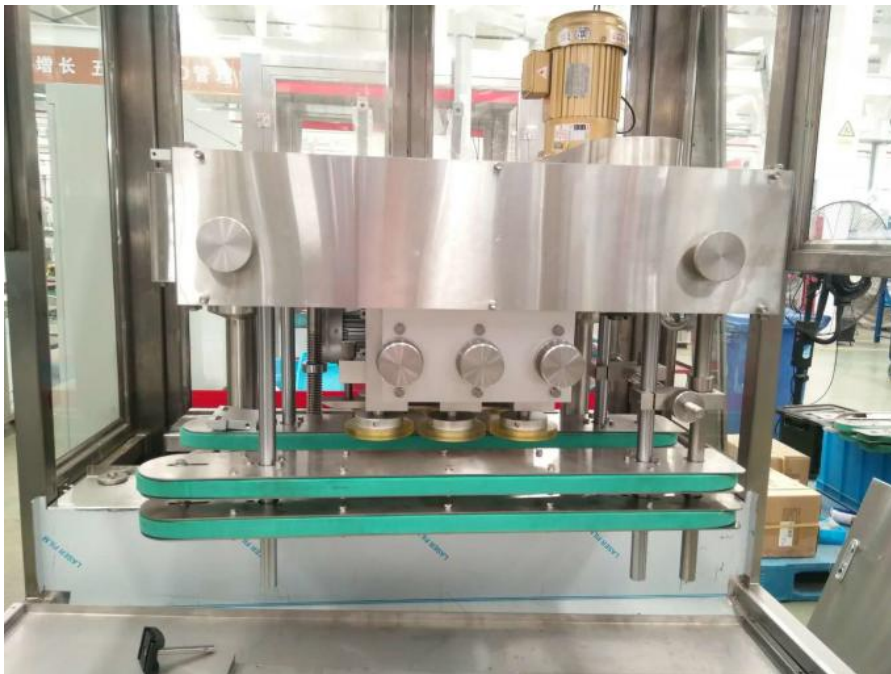
Screwing cap driving part
