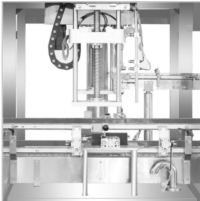
Tool-free quick disconnect for capping heads
