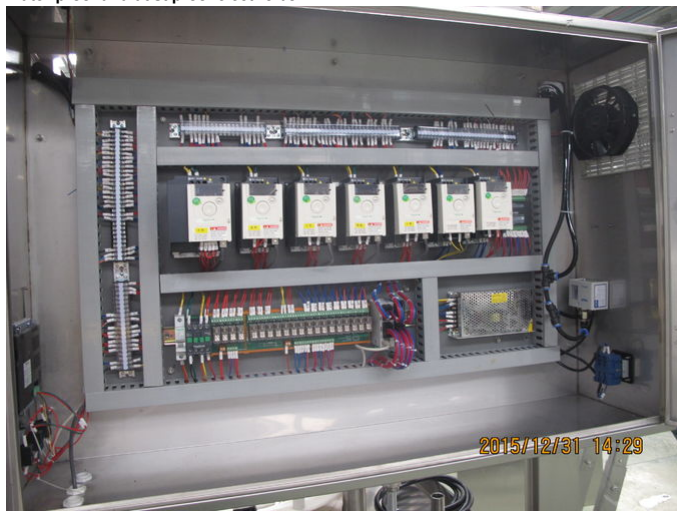
Water-proof and dust proof electric box
