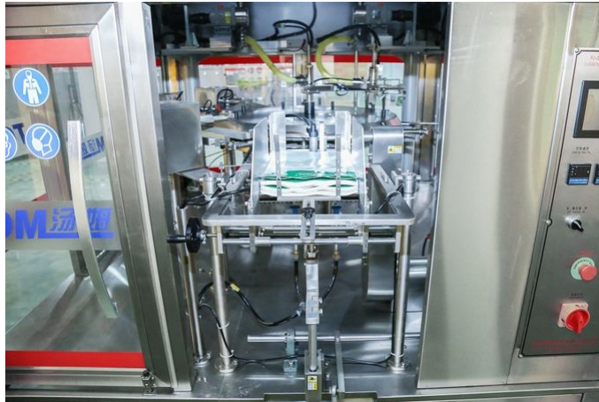
This is the bag outlet conveyor, after filling and sealing, the bag will come out by this conveyor to enter into the next packing station
