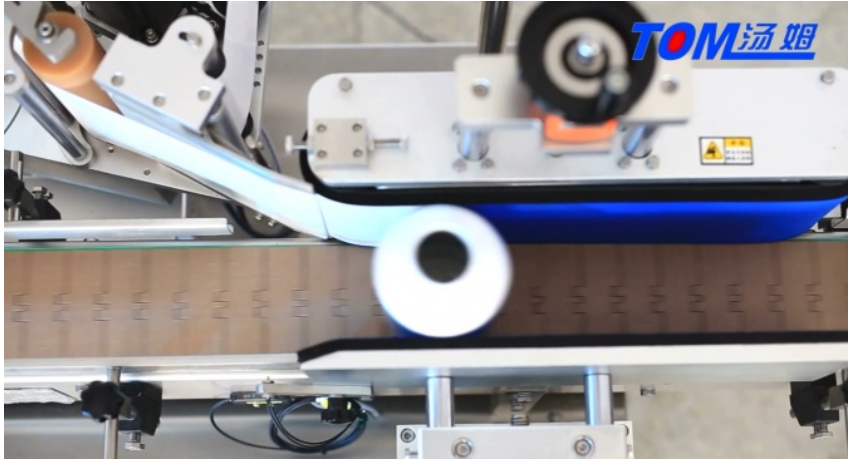
Equipped with label storage place, to prevent the label is distorted, label dispatching and back paper collecting is driven by motor to ensure smooth and accurate label sticking
